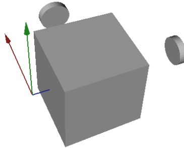
Figure 8: scene view of the diffusing cube and the 2 photodiodes. Viewed by opening the file scene.FCStd with FreeCAD ( https://www.freecad.org ).
