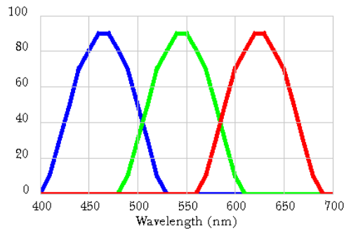
Figure 6: Example of filters for a RGB camera
